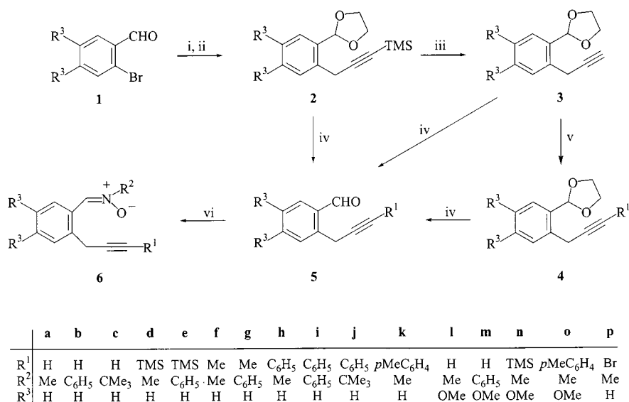
Scheme 3. Reagents: (i) HOCH 2 CH 2 OH, PTSA; (ii) a) n BuLi, b) MgBr 2 , c) BrCH 2 C≡CSiMe 3 ; (iii) Bu 4 NHSO 4 , NH 4 Cl, KF; (iv) PTSA, acetone/H 2 O; (v) ArI, PdCl 2 (PPh 3 ) 2 , CuI, NEt 3 or a) n BuLi, b) CH 3 I; (vi) CH 3 NHOH·HCl, NaOAc or PhNHOH, CH 2 Cl 2
