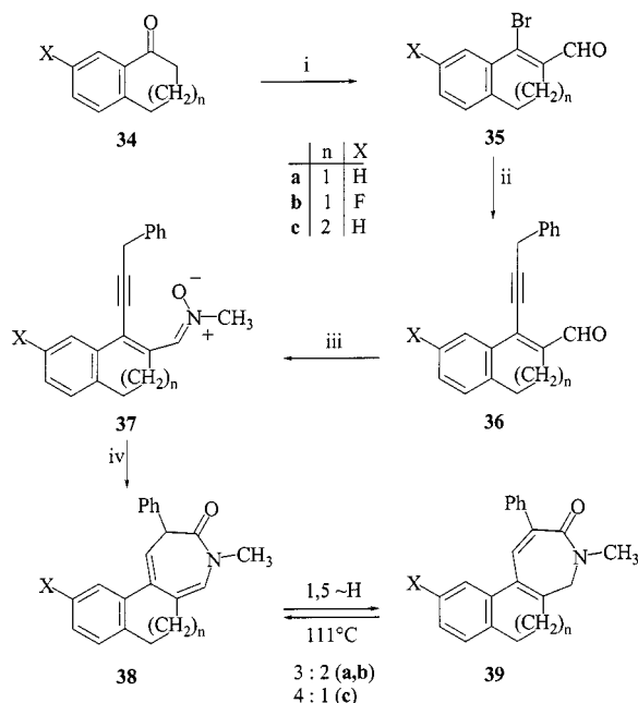
Scheme 13. Reagents: (i) \text{PBr}_3 , DMF, \text{CHCl}_3 ; (ii) \text{HC}\equiv\text{CCH}_2\text{Ph} , \text{PdCl}_2(\text{PPh}_3)_2 , \text{CuI} , \text{K}_2\text{CO}_3 and/or \text{NEt}_3 , \text{C}_6\text{H}_6 ; (iii) \text{CH}_3\text{NHOH}\cdot\text{HCl} , \text{NaOAc} , \text{CH}_2\text{Cl}_2 ; (iv) \text{NaOMe} or \text{KOH} , \text{MeOH}
