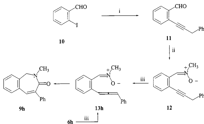
Scheme 6. Reagents: (i) \text{HC}\equiv\text{CCH}_2\text{Ph} , \text{PdCl}_2(\text{PPh}_3)_2 , \text{CuI} , \text{NEt}_3 , \text{C}_6\text{H}_6 ; (ii) \text{CH}_3\text{NHOH}\cdot\text{HCl} , \text{NaOAc} , \text{CH}_2\text{Cl}_2 ; (iii) \text{NaOMe} , \text{MeOH}
