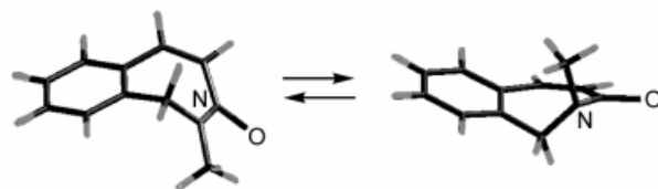
Figure 2. Minimum geometries of 9a calculated with SPARTAN 1.5 (AM1 method)
