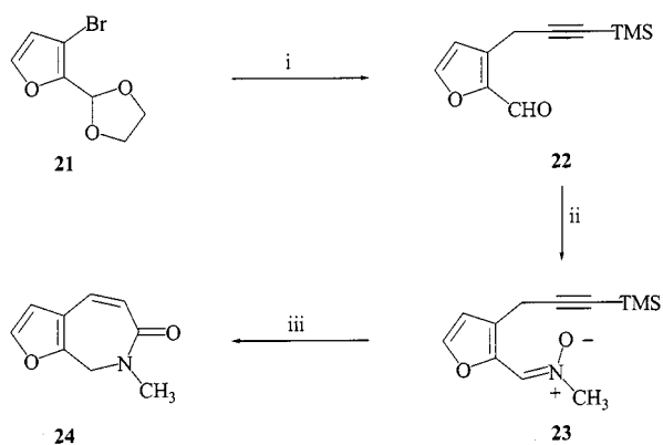
Scheme 10. Reagents: (i) a) n BuLi, b) MgBr 2 , c) BrCH 2 C≡CSiMe 3 , d) PTSA, acetone/H 2 O; (ii) CH 3 NHOH·HCl, NaOAc, CH 2 Cl 2 ; (iii) NaOAc, MeOH
