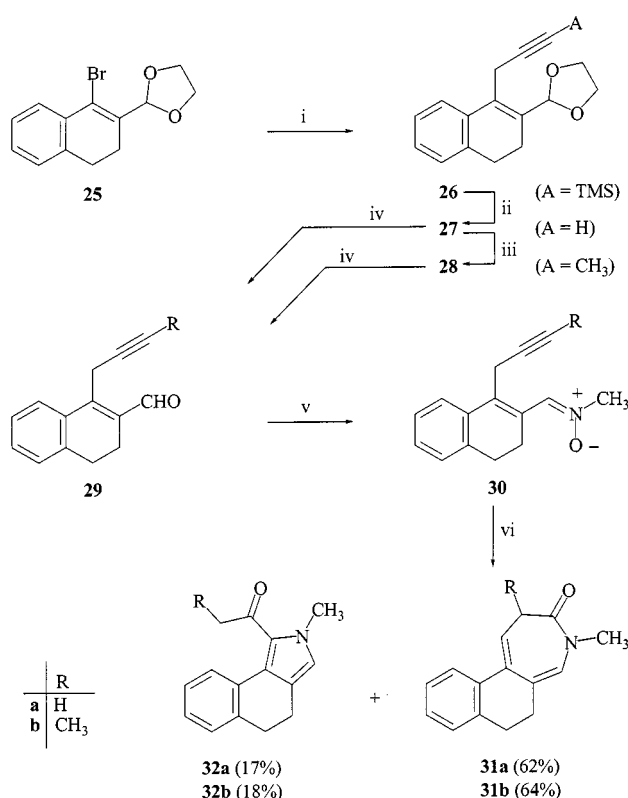
Scheme 11. Reagents: (i) a) n BuLi, b) MgBr 2 , c) BrCH 2 C≡CSiMe 3 ; (ii) K 2 CO 3 , MeOH; (iii) a) n BuLi, b) CH 3 I; (iv) PTSA, acetone/H 2 O; (v) CH 3 NHOH·HCl, CH 2 Cl 2 ; (vi) NaOMe or KOH, MeOH
