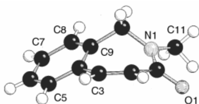
Figure 1. Crystal structure of the benzazepinone 9a (SCHAKAL drawing, hydrogen atoms omitted; the numbering does not correspond with the correct nomenclature); selected bond lengths [Å] and torsion angles [°]: C1–O 1.234, C1–N 1.342, C1–C2 1.480, C2–C3 1.330, C3–C4 1.463, C4–C9 1.394, C9–C10 1.497, C10–N 1.462; C1–C2–C3–C4 -8.8 , N–C1–C2–C3 41.2 , C10–N–C1–C2 4.4 , C9–C10–N–C1 -71.04 , C4–C9–C10–N 67.21 , C3–C4–C9–C10 -3.1 , C9–C4–C3–C2 -30.7 .
